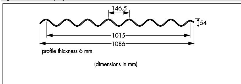
Figure 1 Cemsix – profile and dimensions
